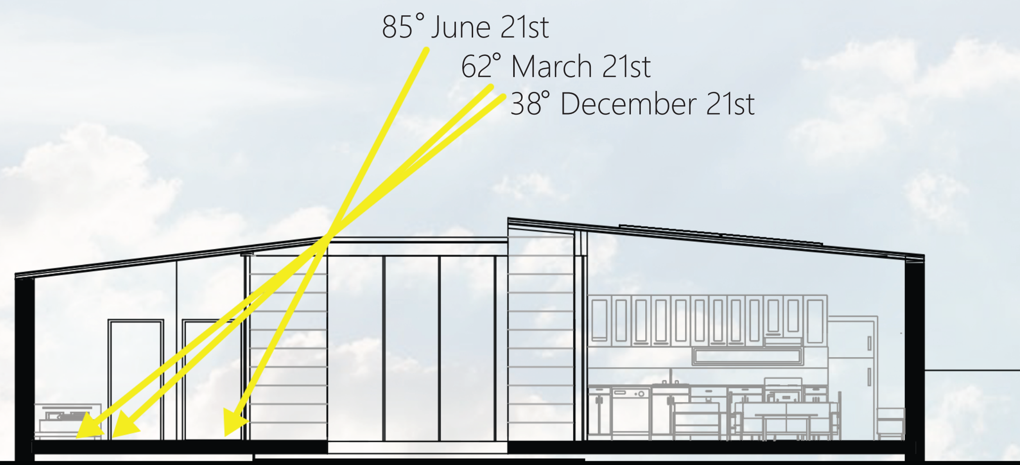
Solar Angles
